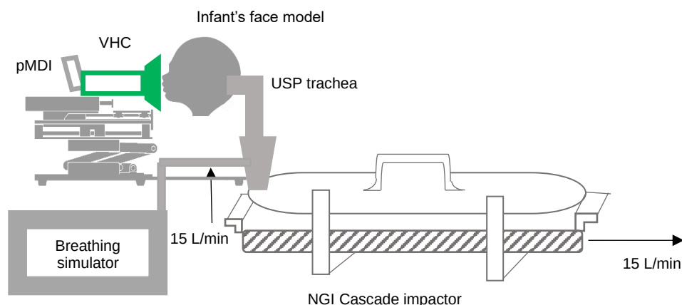
Figure 2 - Schematic drawing of the IIVC bench model for APSD determination.
